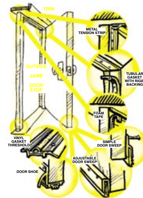
Weatherstripping options for doors
