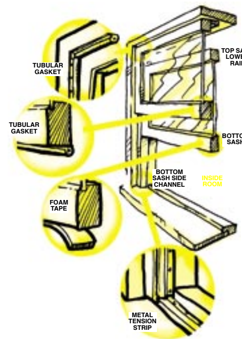
Weatherstripping options for windows
